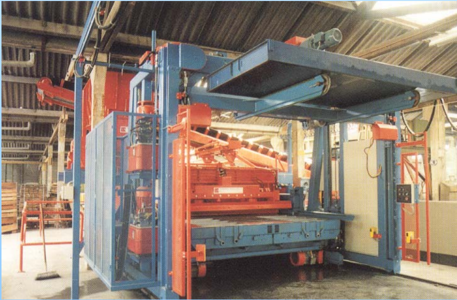
MPF Stationary machine with feedbox and trowelling device
